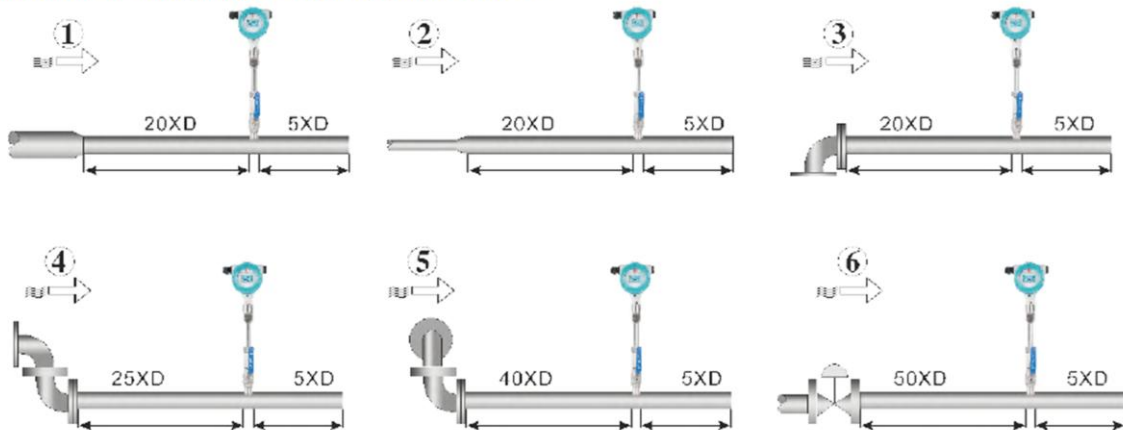
Installation upstream and downstream straight pipe
