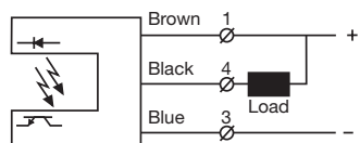
NxS / NP3S Load as NPN
