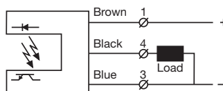
PxS / NP3S Load as PNP
