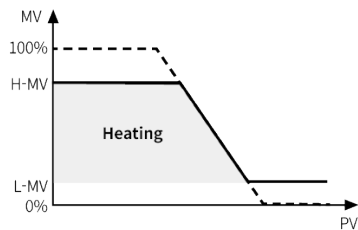
Heating-Cooling control
